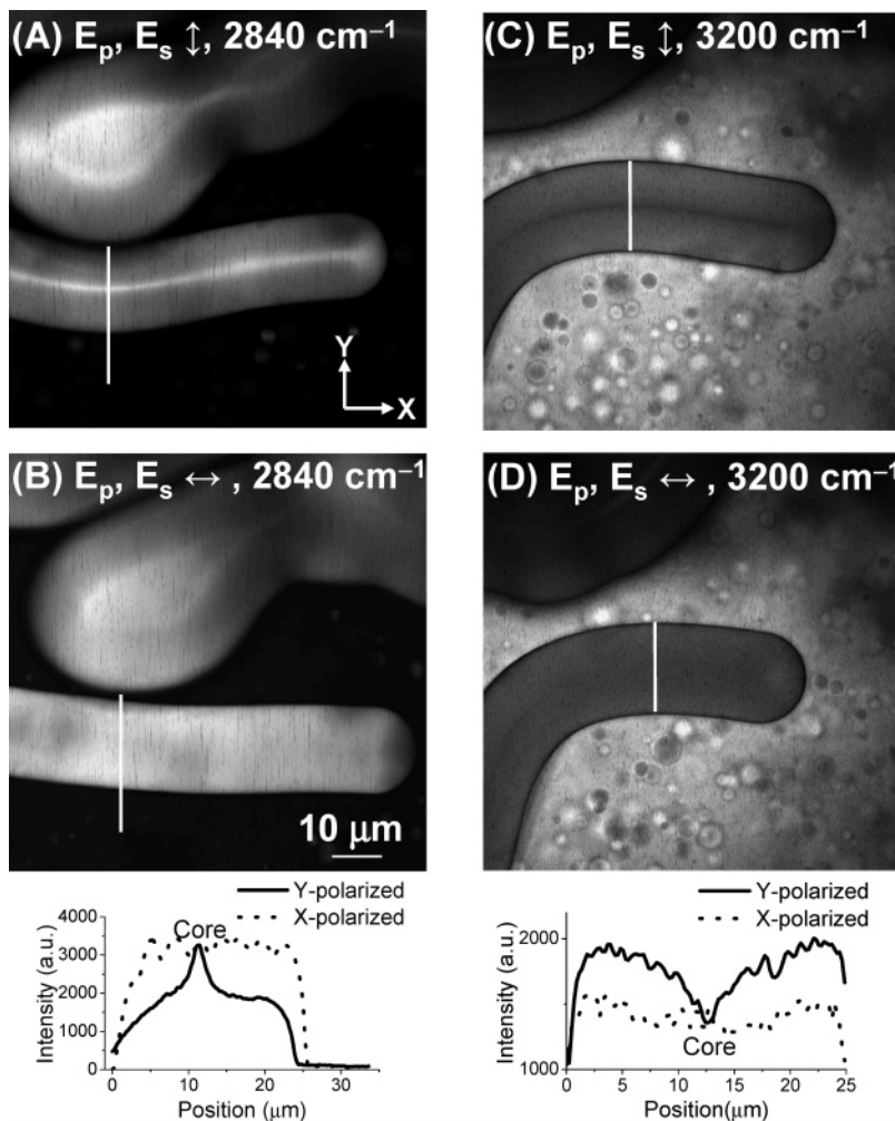
Figure 2. CARS images of C_{12}E_3 myelin figures. \omega_p - \omega_s was tuned to 2840\text{ cm}^{-1} for CH_2 (A and B) and 3200\text{ cm}^{-1} for H_2O (C and D). The polarization direction of the parallel-polarized pump and Stokes beams is marked in each image. Shown below the images are the intensity profiles along the white lines in the images. The pump beam frequency was fixed at 14300\text{ cm}^{-1} . The average power of the pump and Stokes beam at the sample was 4.5 and 2.1 mW, respectively. Similar powers were used for other CARS images. The acquisition time was 2.7 s for each CARS image of 512 \times 512 pixels. Due to their dynamic nature, the myelin figure growth direction changed after 5 min, the time we used to tune \omega_p - \omega_s to 3200\text{ cm}^{-1} . The upper myelin figure is an example of a tadpole.
