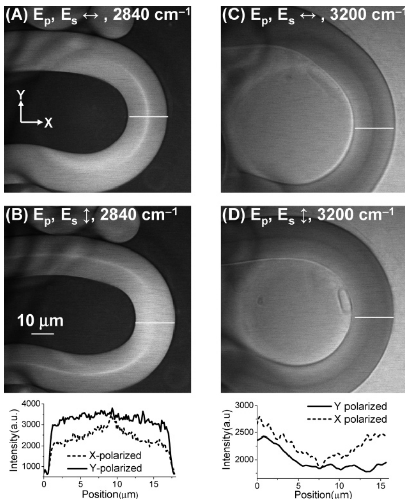
Figure 6. CARS images of AOT myelin figures. \omega_p - \omega_s was tuned to 2840 \text{ cm}^{-1} for \text{CH}_2 (A and B) and 3200 \text{ cm}^{-1} for \text{H}_2\text{O} (C and D). The polarization direction of the parallel-polarized pump and Stokes beams is shown in each image. Notice the large CARS intensity from water in the myelin. Below the images are the intensity profiles along the white lines in the images.
