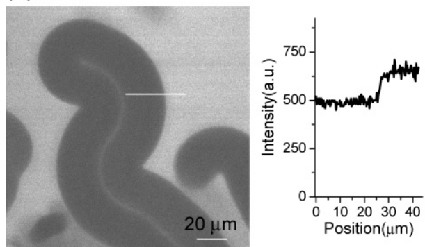
Figure 8. Confocal fluorescence images of C 12 E 3 myelin figures. (A) Signal from DOPE–rhodamine that labels the surfactant bilayers. (B) Signal from FITC that labels the water phase. The intensity profiles along the white lines are shown to the right.
