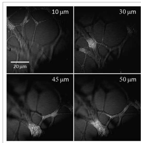
Figure 3. 3-D structure of unstained neurites growing in a 1% CS gel matrix inspected by a laser-scanning CARS microscope. Representative images at different depths show the 3-D distribution of the neurite growth. The number marked in each image indicates the depth relative to the bottom layer of neurite observed in the field of view.
