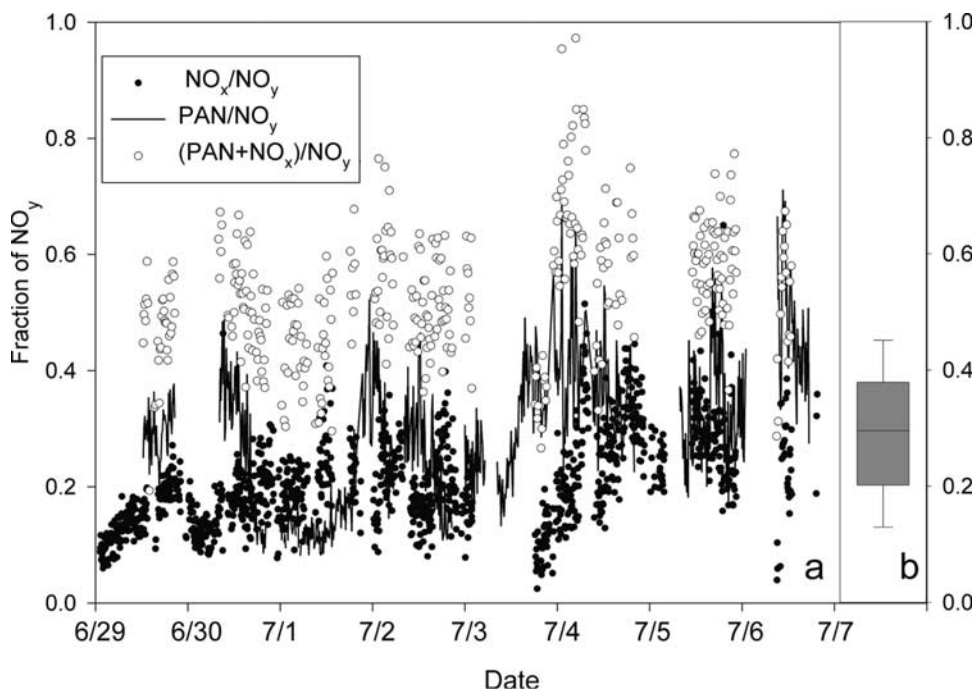
Figure 3. (a) NO x /NO y , PAN/NO y , and (PAN + NO x )/NO y , during Summit 98. (b) Box and whisker plot of PAN/NO y , Summit 98.
