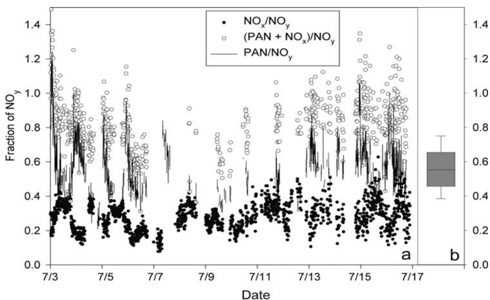
Figure 4. (a) NO x /NO y , PAN/NO y , and (PAN + NO x )/NO y , during Summit 99. (b) Box and whisker plot of PAN/NO y , Summit 99.
