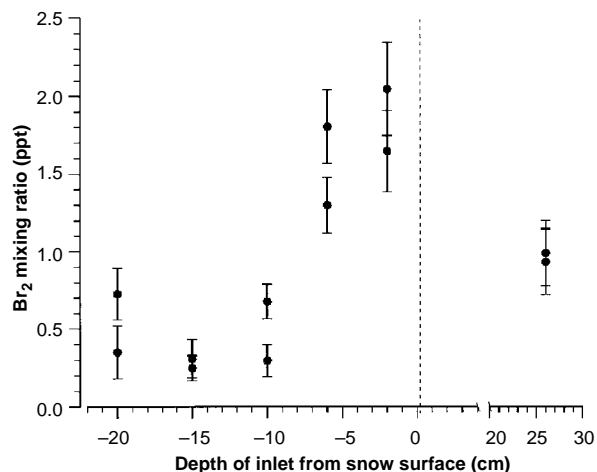
Fig. 2. Br 2 mixing ratios measured with the ion pair 158/79 in snowpack interstitial air and in the air above on day 63 (3 March). Error bars are \pm 2\sigma .
