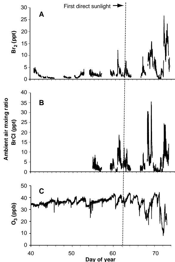
Fig. 1. Ambient mixing ratios of (A) Br 2 with the ion pair 158/79. The same mixing ratios of Br 2 are derived with the 160/79 or 160/81 ion pairs. (B) BrCl with the ion pair 114/35. The same mixing ratios of BrCl are derived with the 116/35 and 116/37 ion pairs. (C) O 3 between days 40 and 73 (9 February to 13 March). The blank areas are periods where calibrations and zeroes were performed or other species were being monitored. Signals were observed for the ion pairs associated with BrCl starting on day 50, but were not above the statistical detection limit until day 54.
