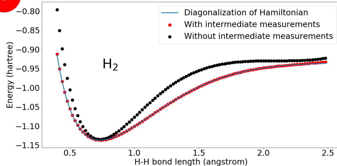
Improved significantly compared to QNN removing intermediate measurements
