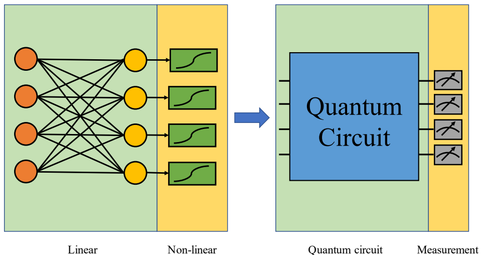
Measurement as the non-linear operation in quantum circuit
