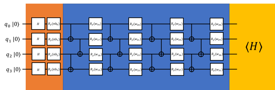
Hybrid quantum neural network to calculate ground state energy
