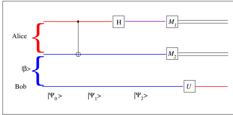
Fig. 1. Quantum circuit for teleporting a qubit. The two top lines represent Alice’s system, while the bottom line is Bob’s system. H represents a Hadamard transformation, M_1 and M_2 represent the measurement on the two top lines.
