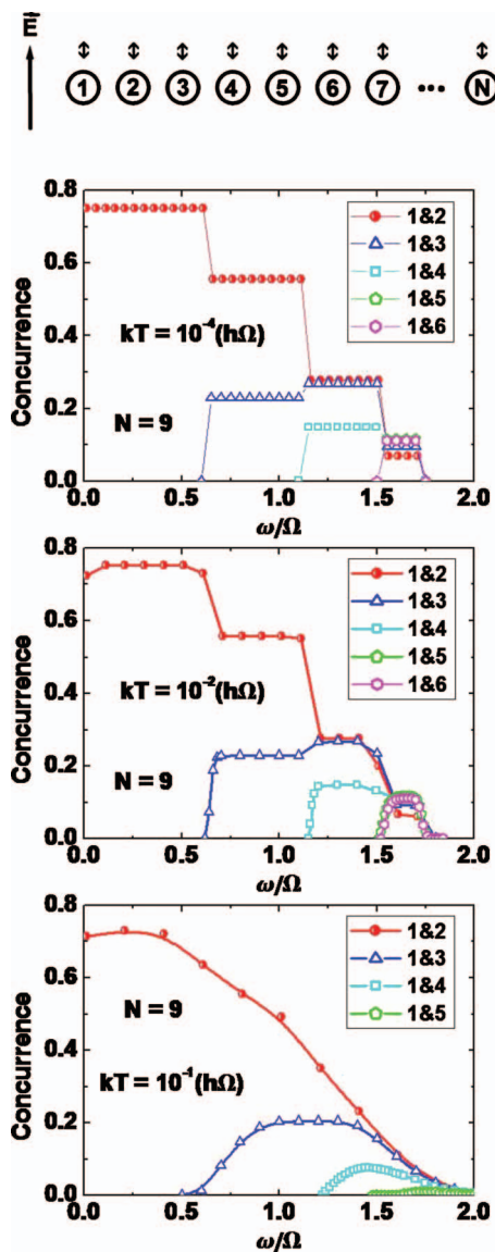
FIG. 1. Pairwise concurrence [Eq. (4)] of one-dimensional arrangements of the dipoles as one varies the ratio \omega/\Omega at kT=10^{-4} , 10^{-2} , and 10^{-1} \hbar\Omega , respectively, for N=9 dipoles.
