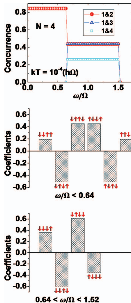
FIG. 2. Pairwise concurrence [Eq. (4)] and coefficients of the wave function of one-dimensional arrangements of the dipoles as one varies the ratio \omega/\Omega at kT=10^{-4} \hbar\Omega for N=4 dipoles.
