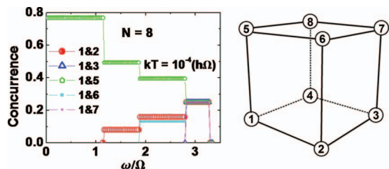
FIG. 4. Pairwise concurrence [Eq. (4)] of three-dimensional simple cubic arrangements of the dipoles as one varies the ratio \omega/\Omega at kT=10^{-4} \hbar\Omega . Here \Omega is the dipole-dipole coupling constant between dipole 1 and dipole 2, \Omega=\Omega_{12} . The external electric field is along dipoles 1 to 5.
