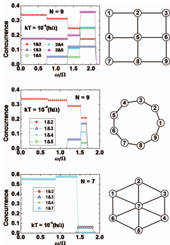
FIG. 3. Pairwise concurrence [Eq. (4)] for different two-dimensional arrangements of the dipoles as one varies the ratio \omega/\Omega at kT=10^{-4} \hbar\Omega . The external electric field is perpendicular to the 2- d plane.
